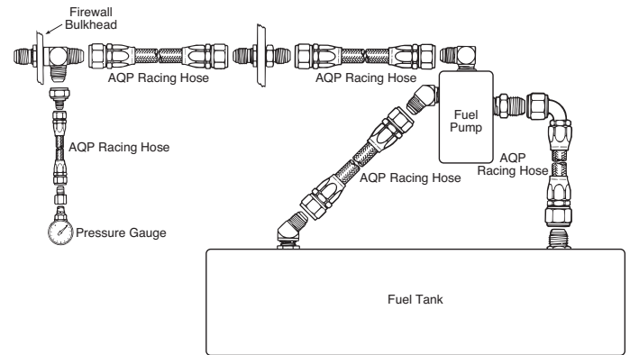
Typical Fuel System Schematic
