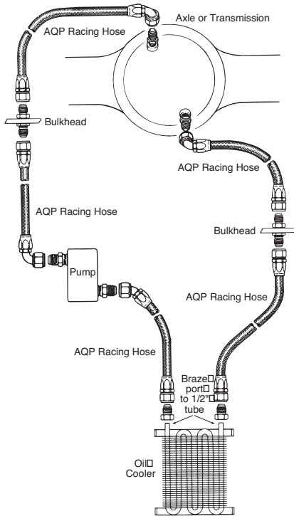
Typical Transmission or Axle Cooler Schematic
