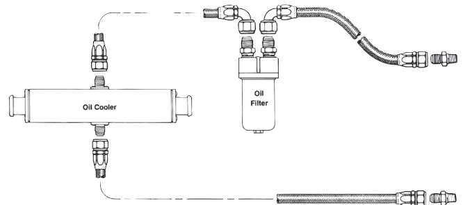
Typical Oil Cooler Schematic
