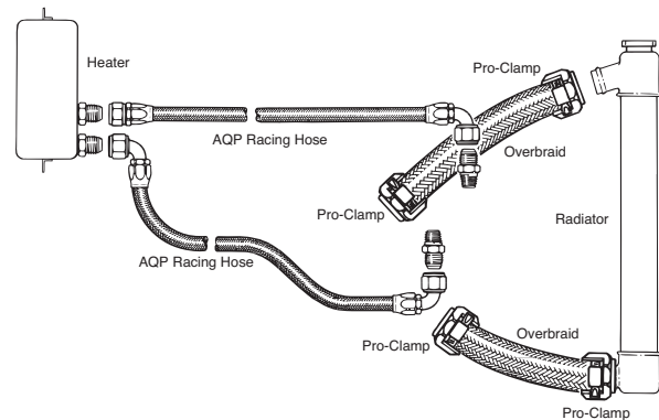
Typical Radiator and Heater Schematic
